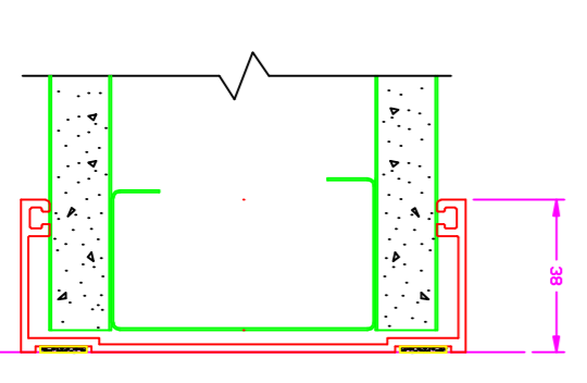
Section Q-Q
