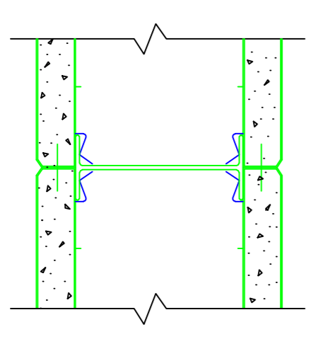
Section P-P
