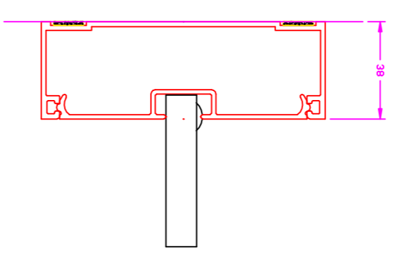
Section H-H
