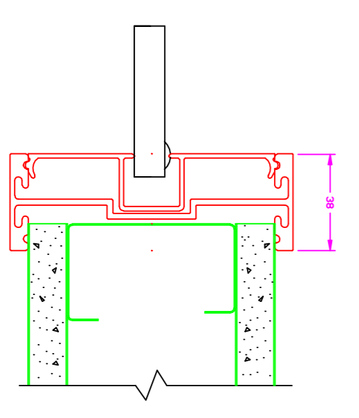
Section N-N
