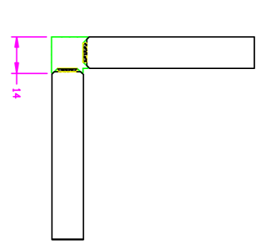
Detail R
